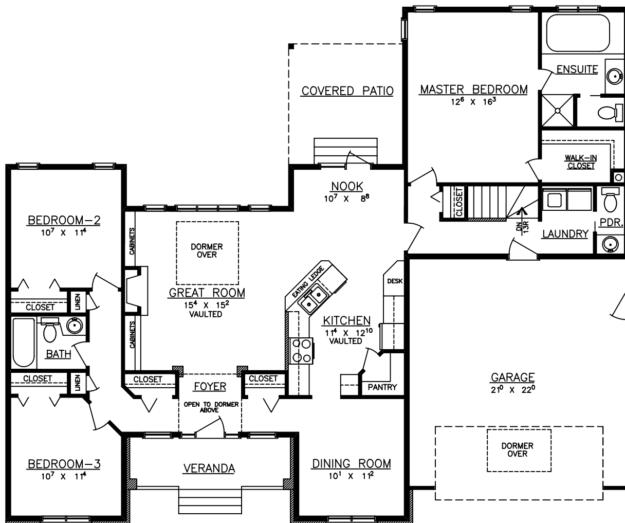
FLOOR PLAN
